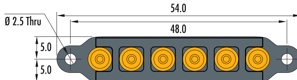
Spring contact back view
